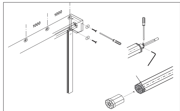
10 Fit the shutter box using the recommended fixings and spacings. Once the shutter box has been installed check the dummy end making sure that it is securely located within the axle. If the dummy end is a shaft bolt design make sure that the centre shaft is fixed in place so that it can not slide back into the axle.
