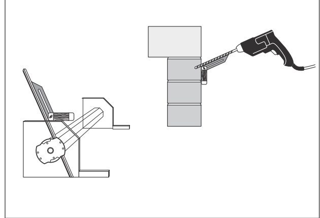
6 If a manual override has been supplied and if applicable determine the angle of the override hole.
