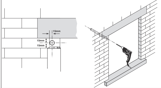
5 If applicable mark and drill the override hole ensuring the hole is drilled at the correct angle (see step 6). Drill a 10mm pilot hole followed by a 22mm hole Tip – hold a block of wood against plaster to reduce damage caused by the drilling process
