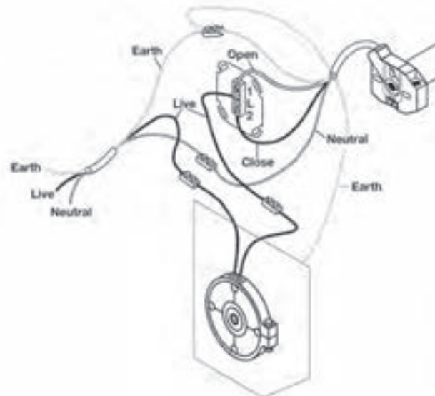
Wiring a safety brake into a circuit with a motor and a standard switch
