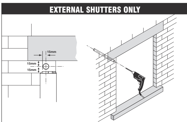
EXTERNAL SHUTTERS ONLY 5 Mark and drill the belt tube hole. Drill a 10mm pilot hole followed by a 22mm hole for the tube. Tip – hold a block of wood against plaster to reduce damage caused by the drilling process.
