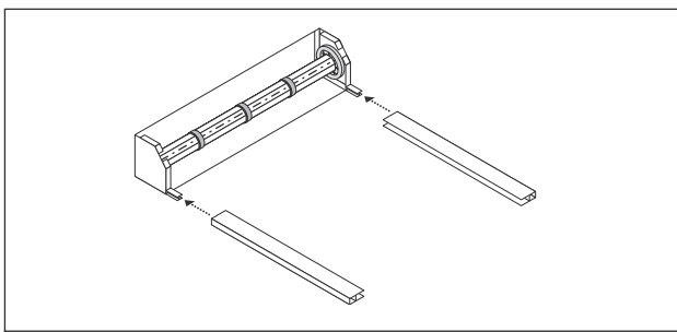
3 Carefully locate the guide rails onto the box lugs ensuring that on face fit guides the 13mm holes are on the outside. The guide rails should have a protective steel guide foot located at the base of each guide rail. When moving the shutter as a complete unit you should take care to prevent the lugs being snapped off the box ends by the leverage available from the guide rails. If the shutter is too large to be lifted up as a complete unit you should offer up, locate and fix the individual guide rails then the shutter box.
