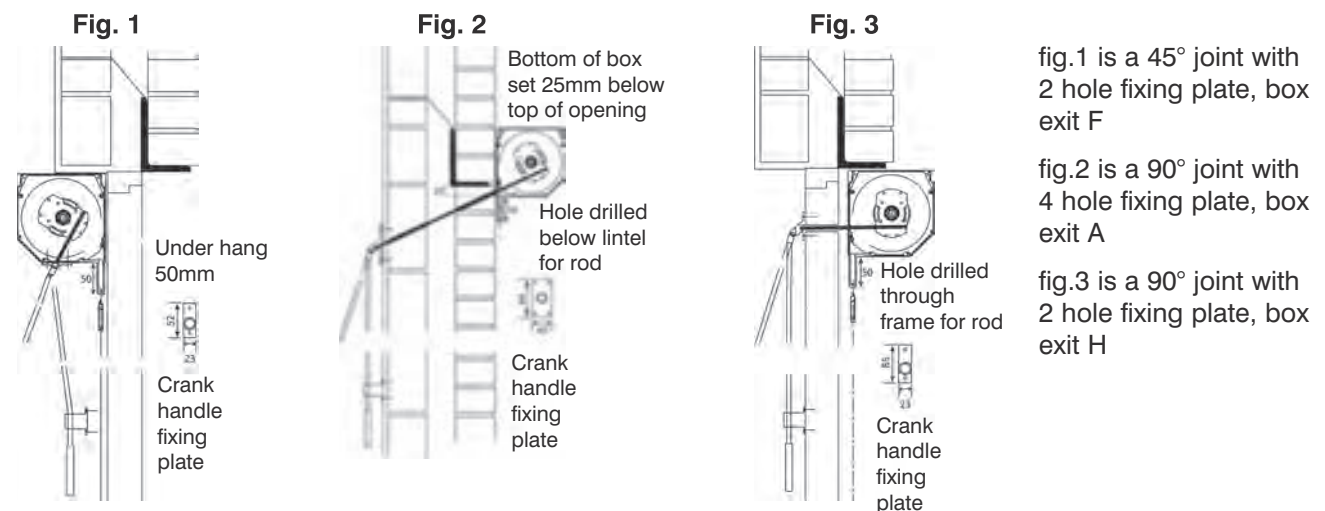
Rigid Eye Joint
