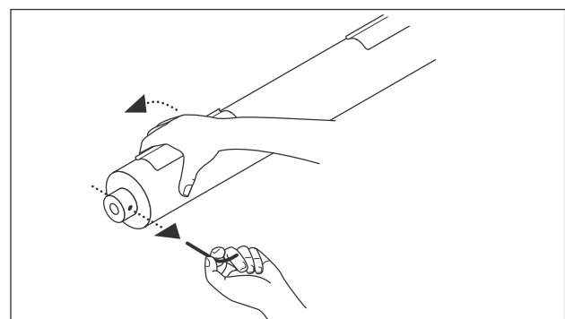
⚠ RISK OF PERSONAL INJURY! 12 Turn the axle in the down direction and carefully remove the pin. Please note there maybe tension on the spring, which will cause the axle to turn.
