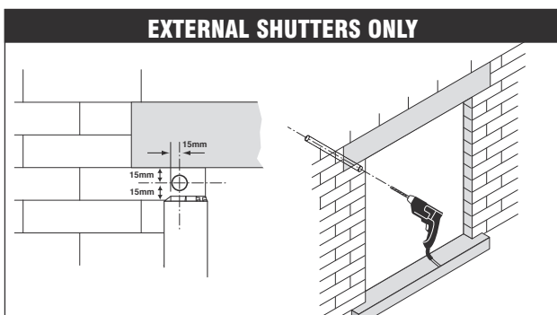
5 Mark and drill the rod crank hole. Refer to step 6 to determine the angle of the crank hole. Please note the shutter box is not shown in this diagram. The location of the hole is determined by the exit hole in the shutter box. Drill a 10mm pilot hole followed by a 22mm hole for the tube.
